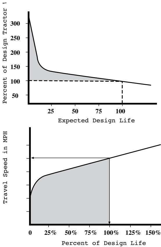
Figure 2. Design life of final drives is reduced with extra ballast and overfueling the engine (top graph). The reduction is a result of overloading the design requirements of the tractor. The major component that determines the design life of a final drive is the tractor’s operating speed (bottom graph). Few final drives are designed to operate at maximum power in the lowest transmission gears.
