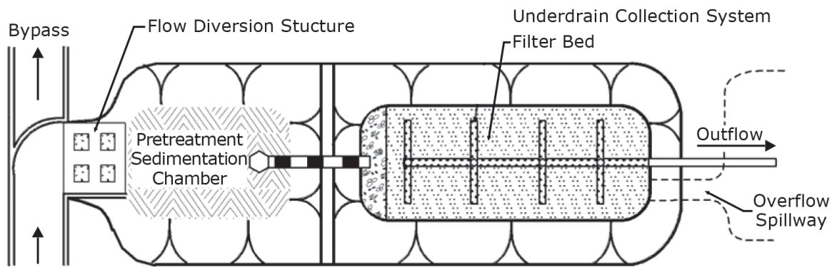
Figure 2. Plan view of typical filtration practice.
